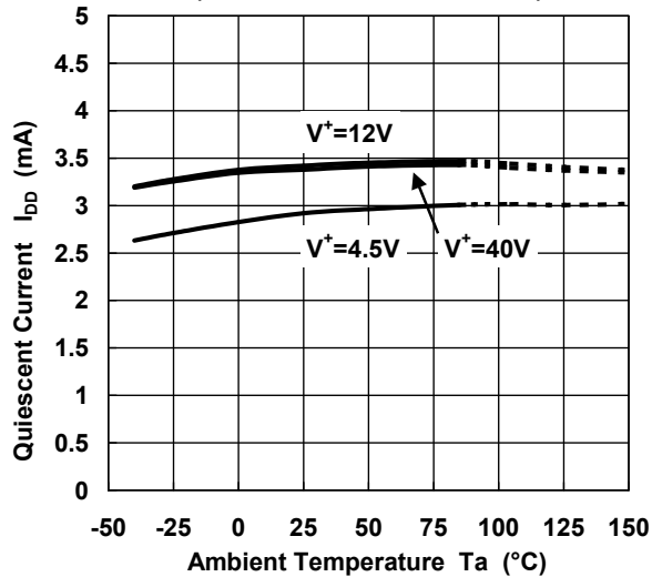
Quiescent Current vs. Temperature (B ver., R_L=no\ load , V_{IN}=0.7V )
