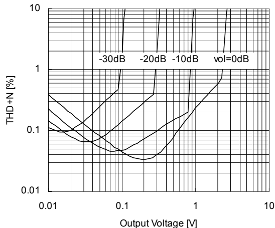
THD+N vs Output Voltage V_+=9V, V_{in}=I_{Na}, f=1\text{kHz}, T_a=25^\circ\text{C} R_g=600\Omega, BW=400\text{Hz}-30\text{kHz}, V_o=OUTa
