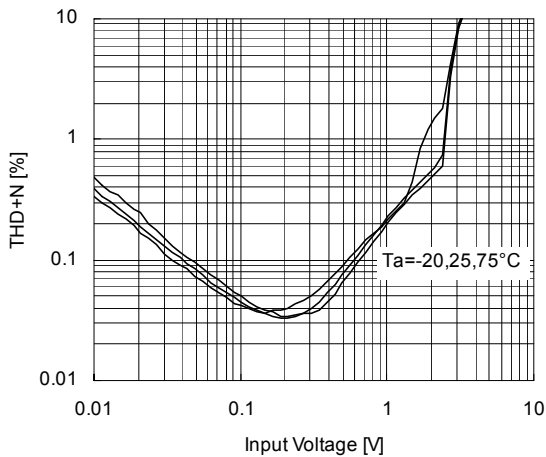
THD+N vs Input Voltage V_+=9V, V_{in}=I_{Na}, f=1\text{kHz}, \text{volume}=0\text{dB} R_g=600\Omega, BW=400\text{Hz}-30\text{kHz}, V_o=OUTa
