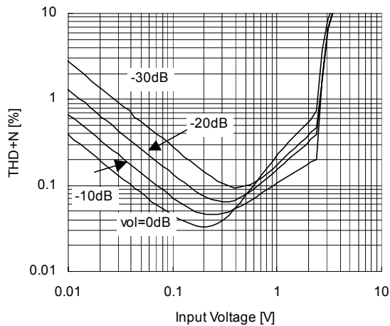
THD+N vs Input Voltage V_+=9V, V_{in}=I_{Na}, f=1\text{kHz}, T_a=25^\circ\text{C} R_g=600\Omega, BW=400\text{Hz}-30\text{kHz}, V_o=OUTa
