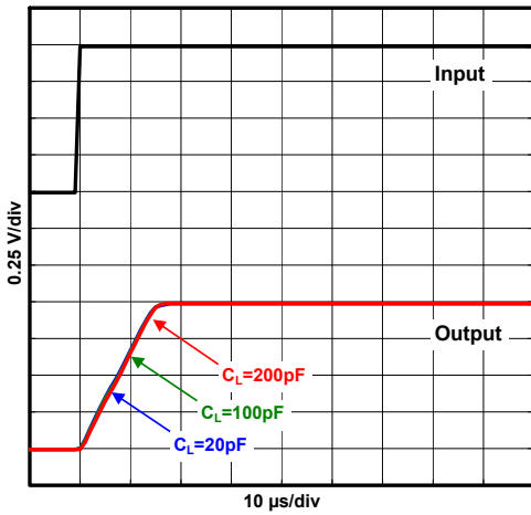
Transient Response
