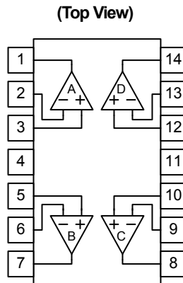
NJM2902CG/NJM2902CAG
