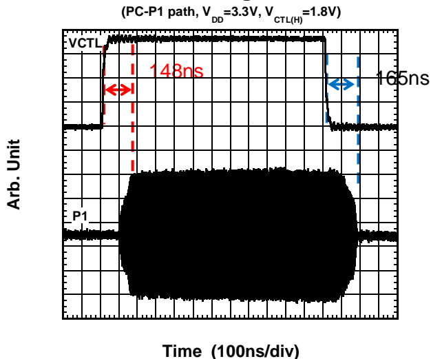
Switching Time
