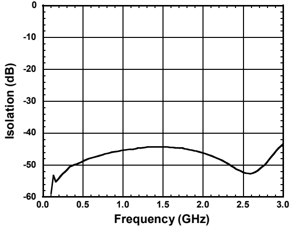
PC-P1 Isolation vs. Frequency ( VCTL1=2.7V, VCTL2=0V, Pin=0dBm )
