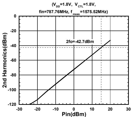
2nd Harmonics
