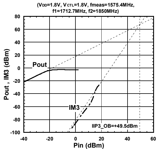
Out-of-band IIP3
