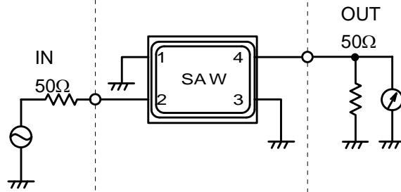
Fig.1 Measuring circuit
