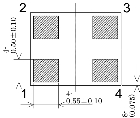
Fig.2 Package dimensions (in mm)
