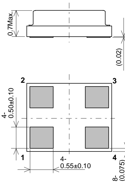
Fig.2 Package dimensions (in mm)
