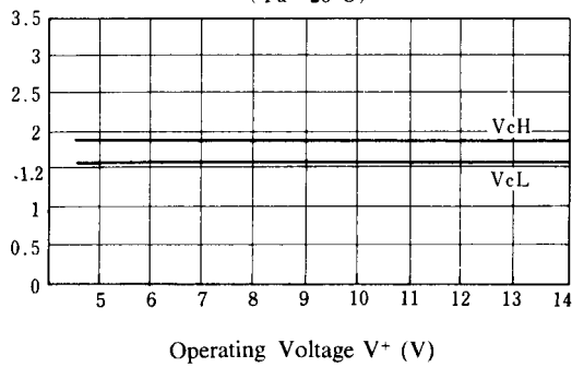
Switch Change Over 1 vs. Operating Voltage ( T_a = 25^\circ\text{C} )
