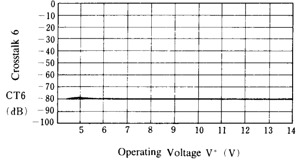
Crosstalk 6 vs. Operating Voltage V^+ (V) ( T_a = 25^\circ\text{C} )
